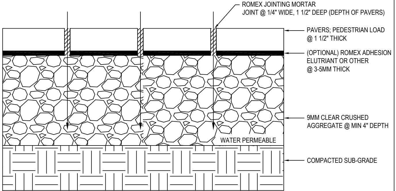
SECTION VIEW
