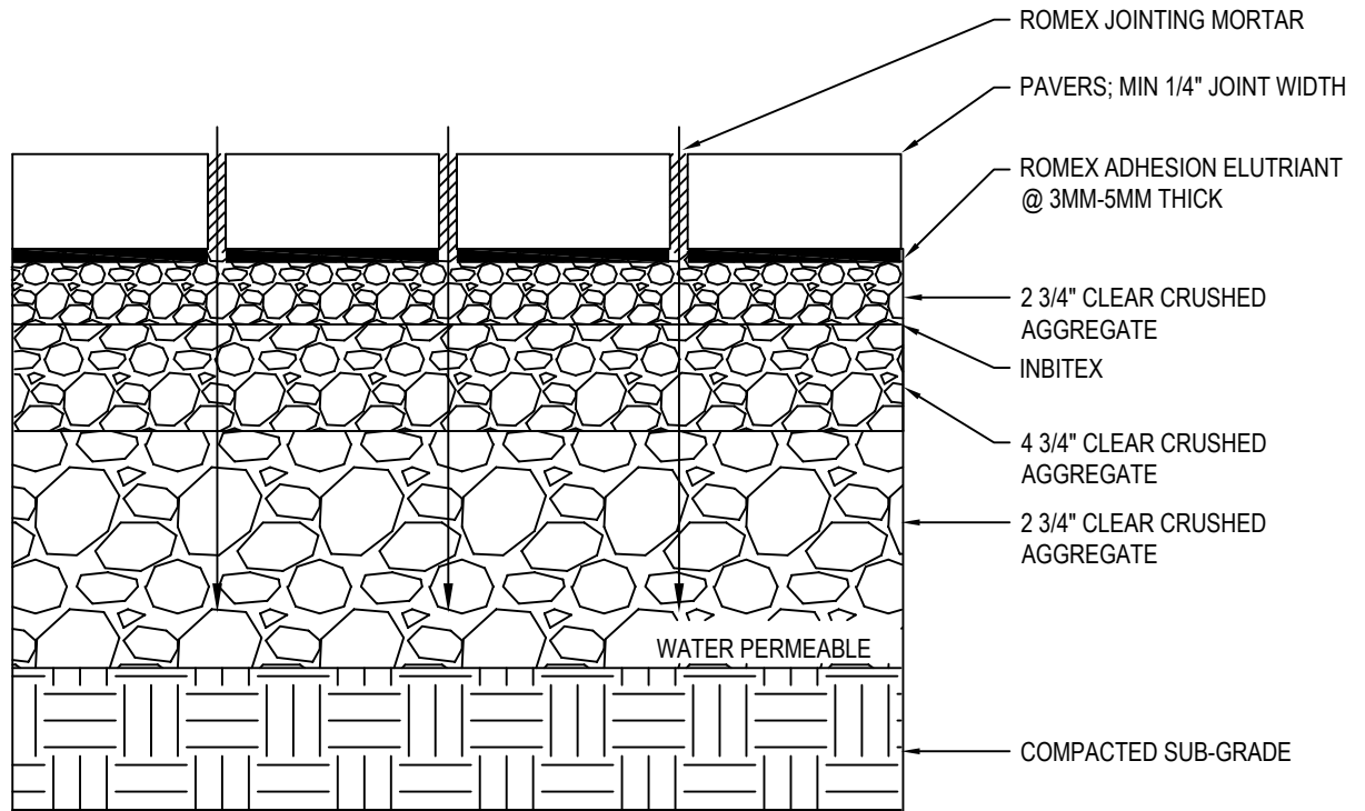
SECTION VIEW
