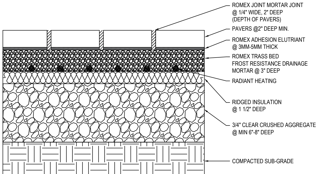
SECTION VIEW
